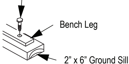
GROUND SILL ATTACHMENT
